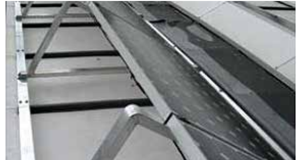
Picture 2: ICB - SOLAFIX as a base for photovoltaic panels
